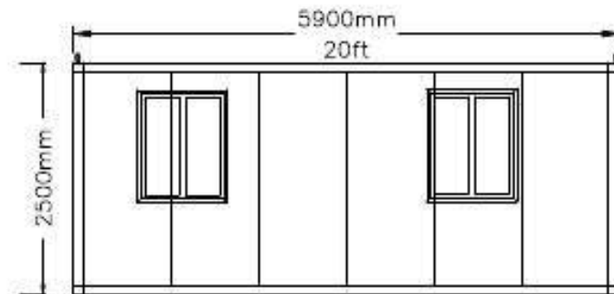
Left view
